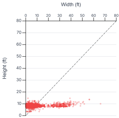
Wall Aspect Ratio
